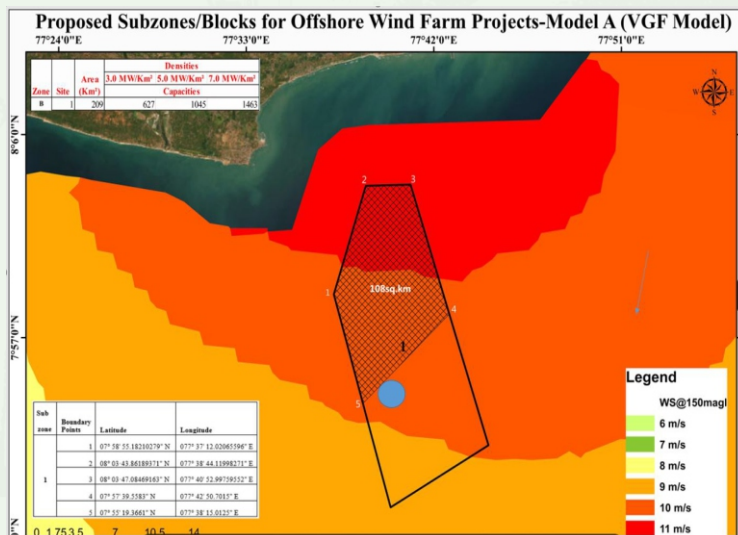
Location of floating buoy with offshore LIDAR
