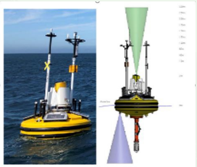
Integrated Floating Wind Lidar
